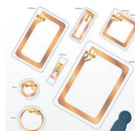
SMAR TLABEL Anti-Counterfeit 13.56MHz chip ISO 14443 A/15693, up to 50 tags(reader/antenna dependent)
