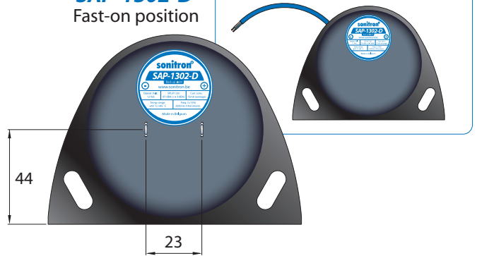
Cable version Standard cable length: 30 cm
