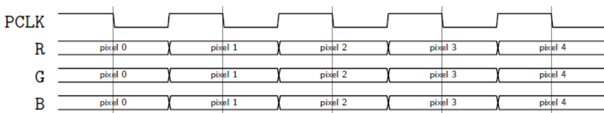
Figure 4: Pixel clocking with no CSPREAD
